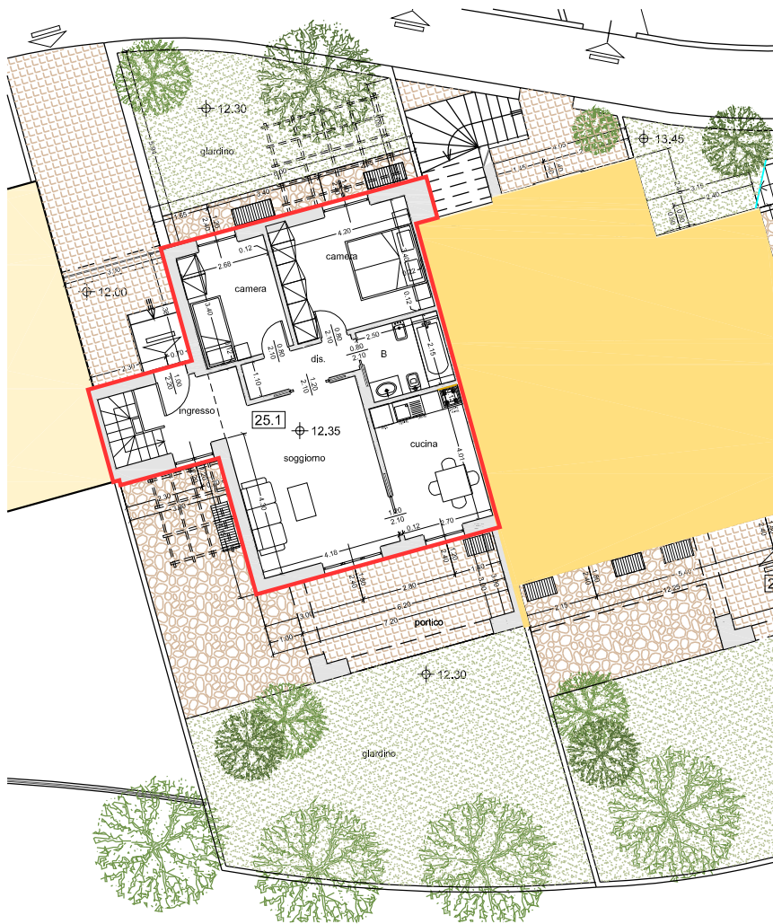
PIANO TERRA
